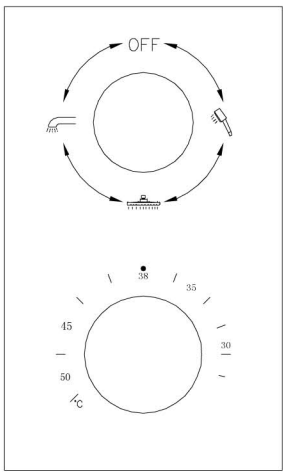
Diverter Function
