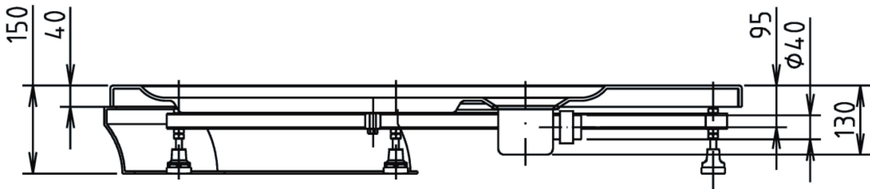
instalace s panelem
