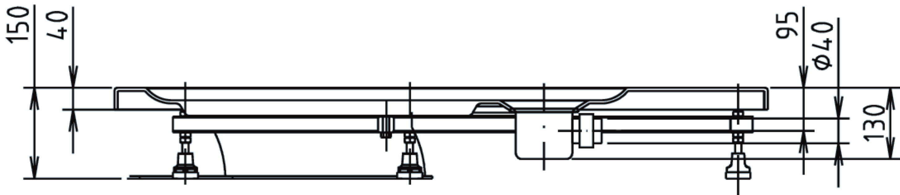
instalace bez panelu
